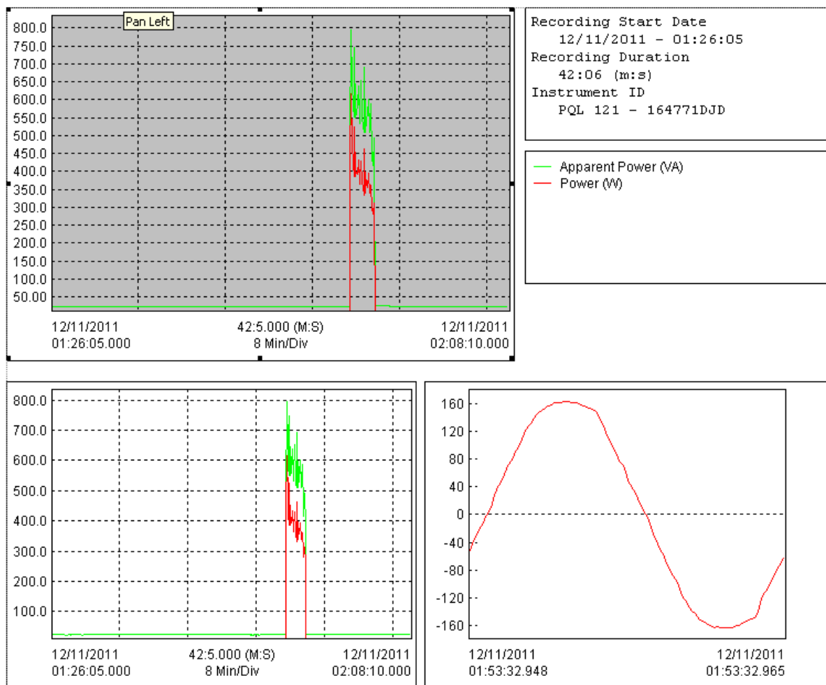
Figure 29 Active power, apparent power, voltage and current RMS of Fan
