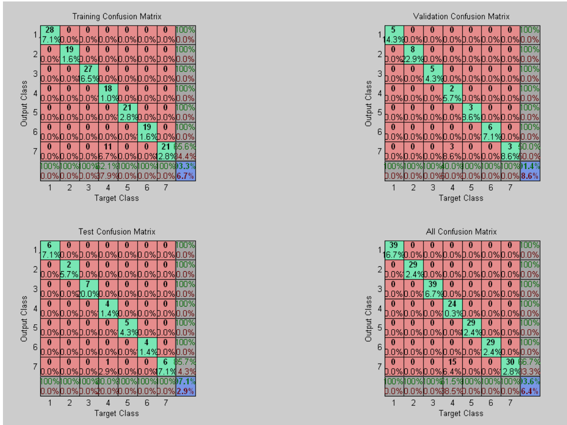
Figure 37 confusion Matrix
